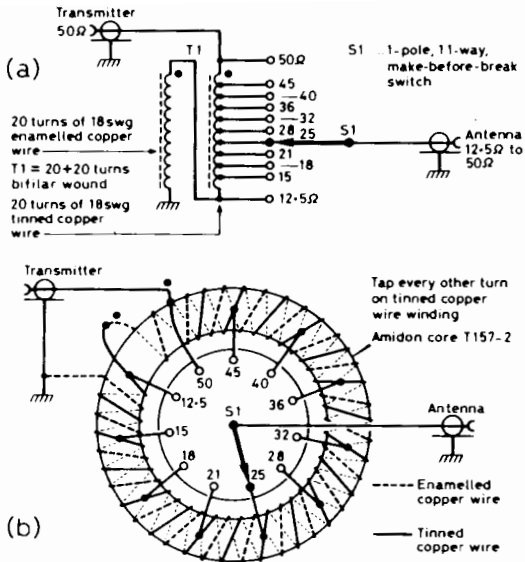
Fig 9. (a) Toroidal matching transformer. (b) Winding layout
